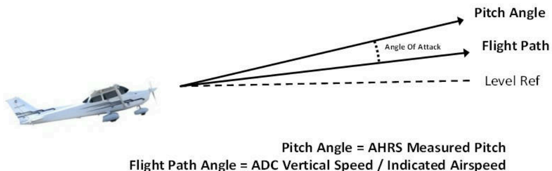
Figure 62: AoA Computation
