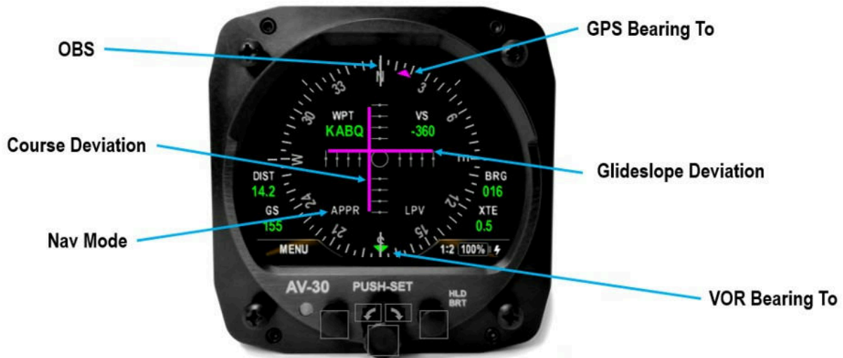
Figure 52: CDI Mode with GPS Guidance
