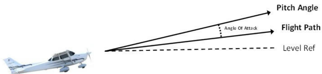
Figure 24: AoA Computation
