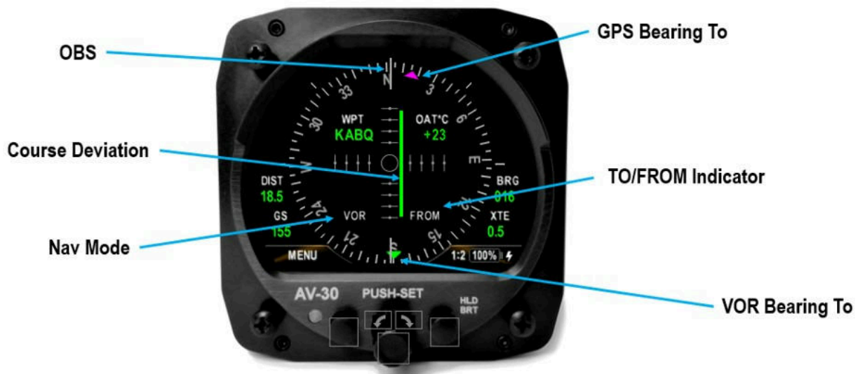
Figure 53: CDI Mode with VOR Guidance
