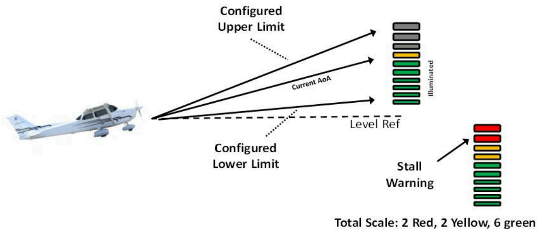
Figure 63: AoA Upper and Lower Limits
