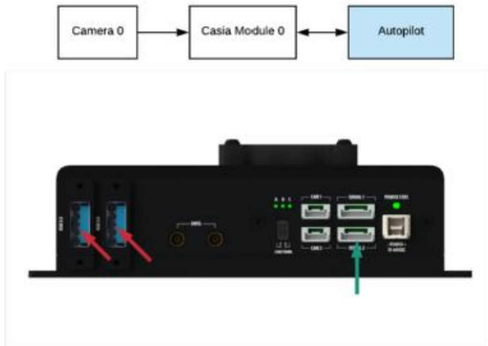
Figure 14: Casia I Data Wiring
