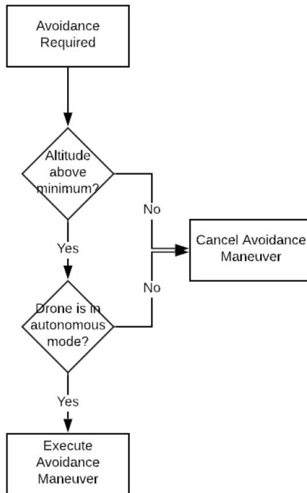
Figure 42: Flow-Chart for Safety Interlocks
