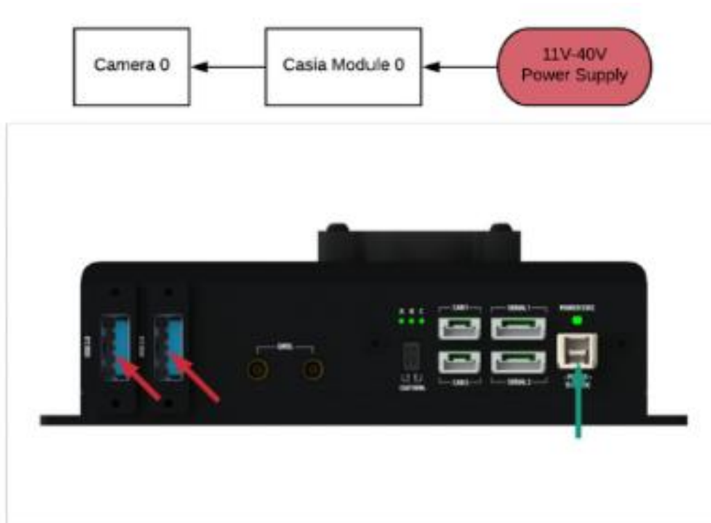
Figure 13: Casia I Power Wiring
