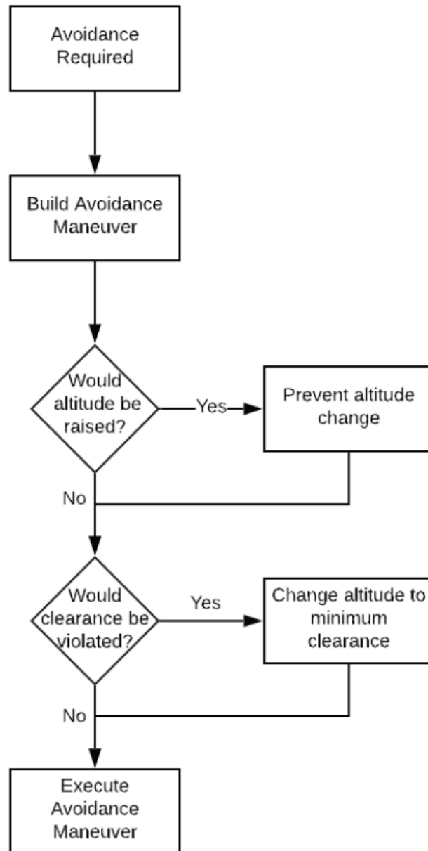
Figure 43: Avoidance Maneuver Logic Flowchart
