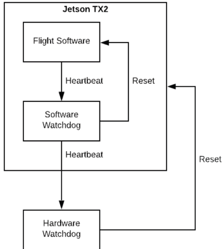
Figure 54: Watchdog Reset and Recover Flowchart
