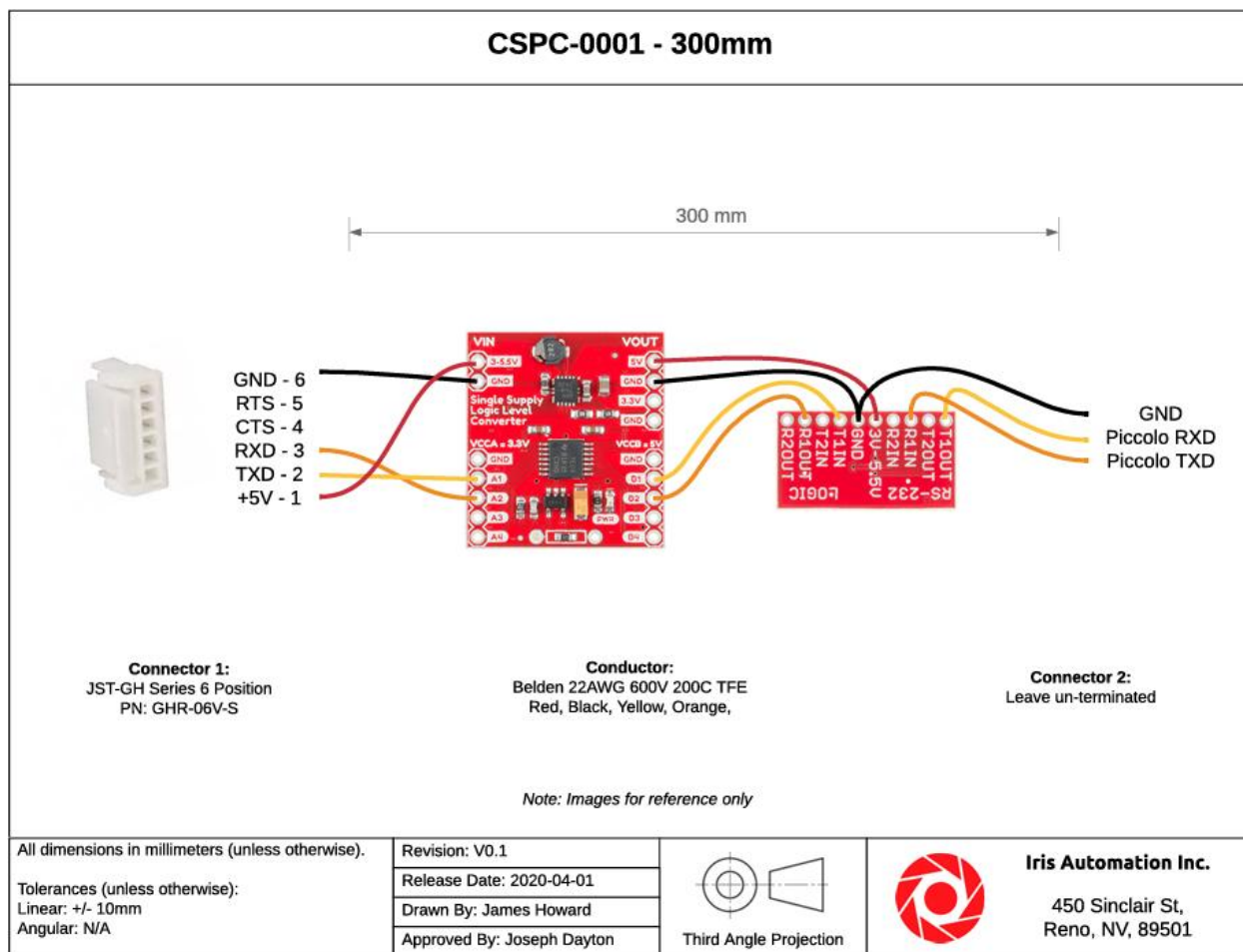
Figure 32: Piccolo RS-232 Converter Wiring Diagram
