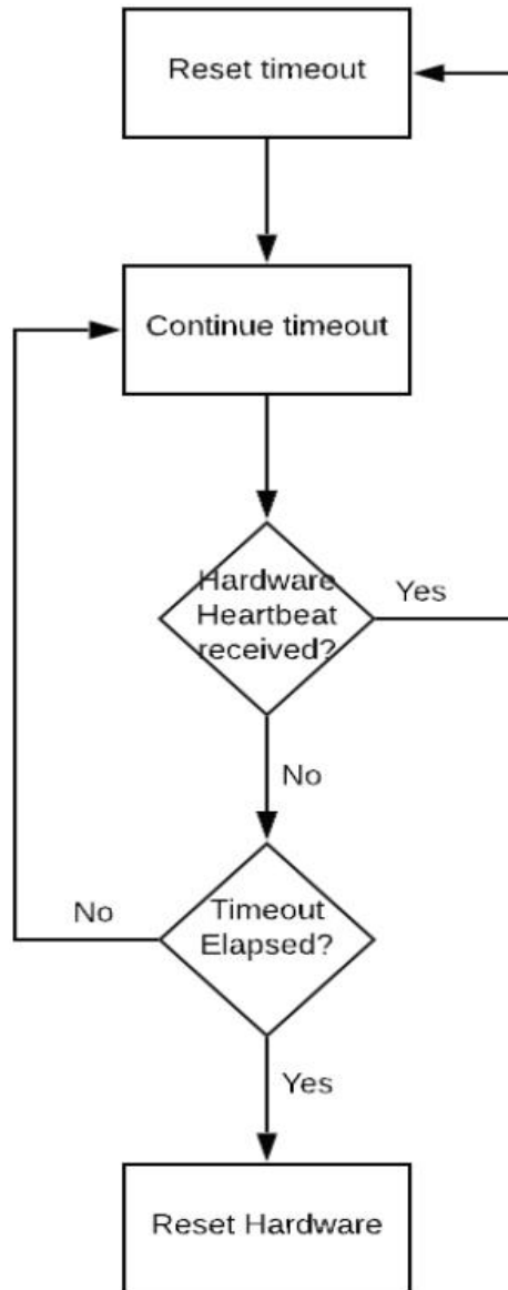
Figure 56: Hardware Watchdog Reset Logic Flowchart
