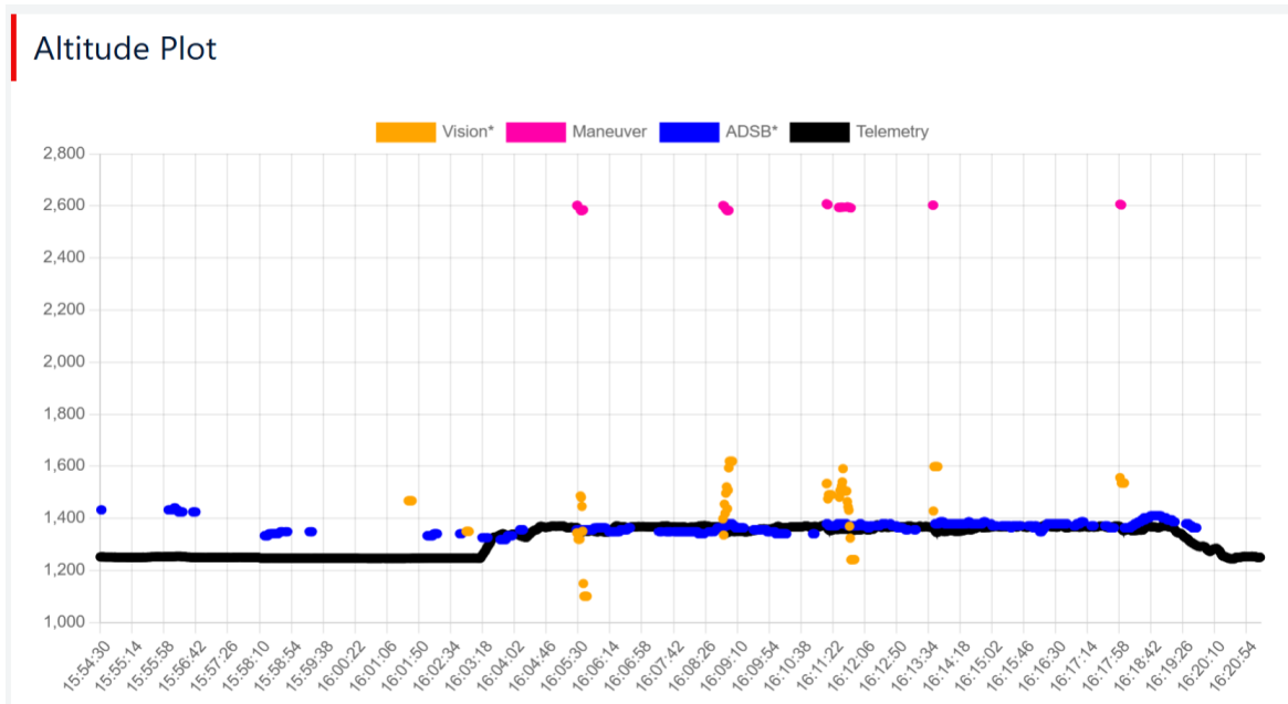
Figure 24: Casia I Altitude Plotter Example
