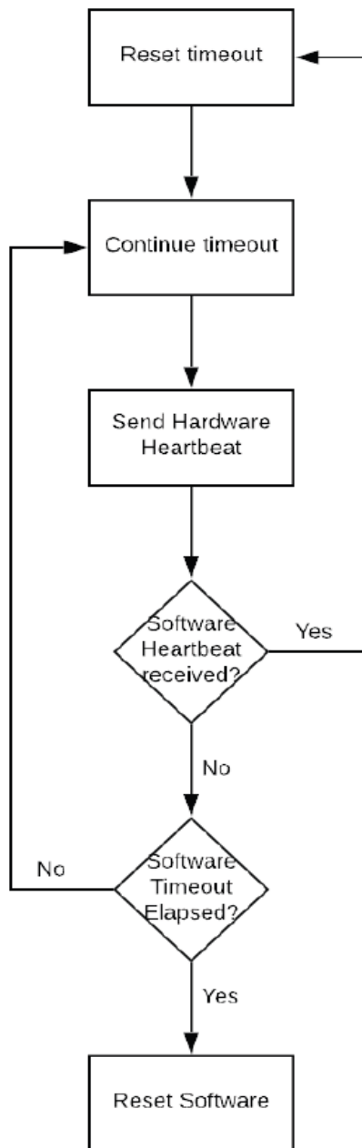
Figure 55: Software Watchdog Reset Logic Flowchart
