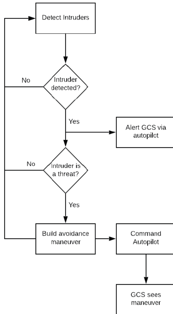
Figure 43: Diagram of Initiating an Avoidance Maneuver
