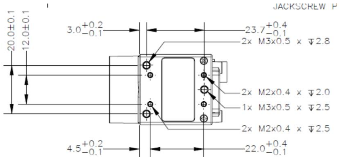
Figure 12: Cameras Mounting Hole Pattern for Casia I
