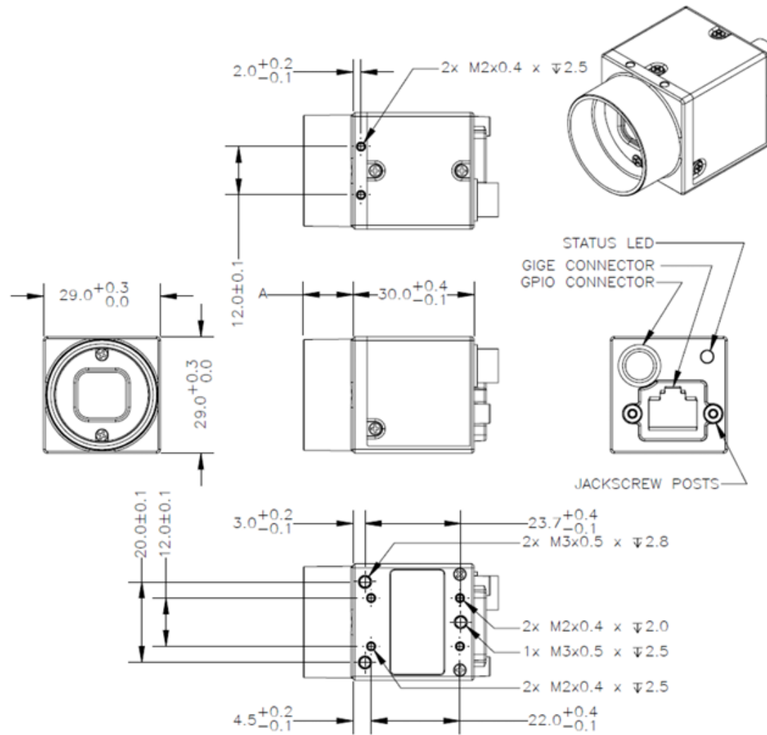
Figure 58: Camera Body FLIR Blackfly S footprint and mount points
