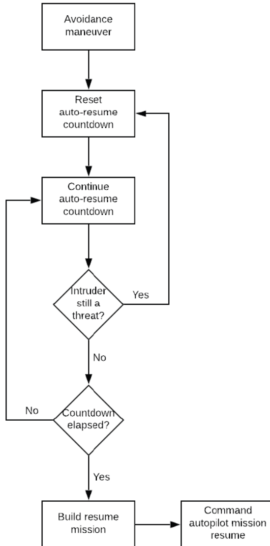
Figure 41: Flowchart for Exiting an Avoidance Maneuver Automatically
