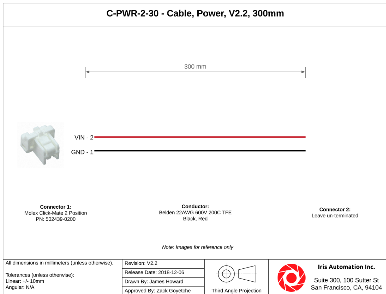
Figure 4: C-PWR-2-30- Cable, Power
