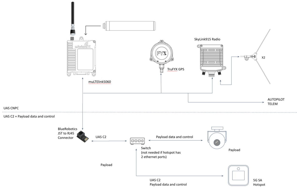
Figure 26: muLTElink Wiring Diagram with Two External Radios
