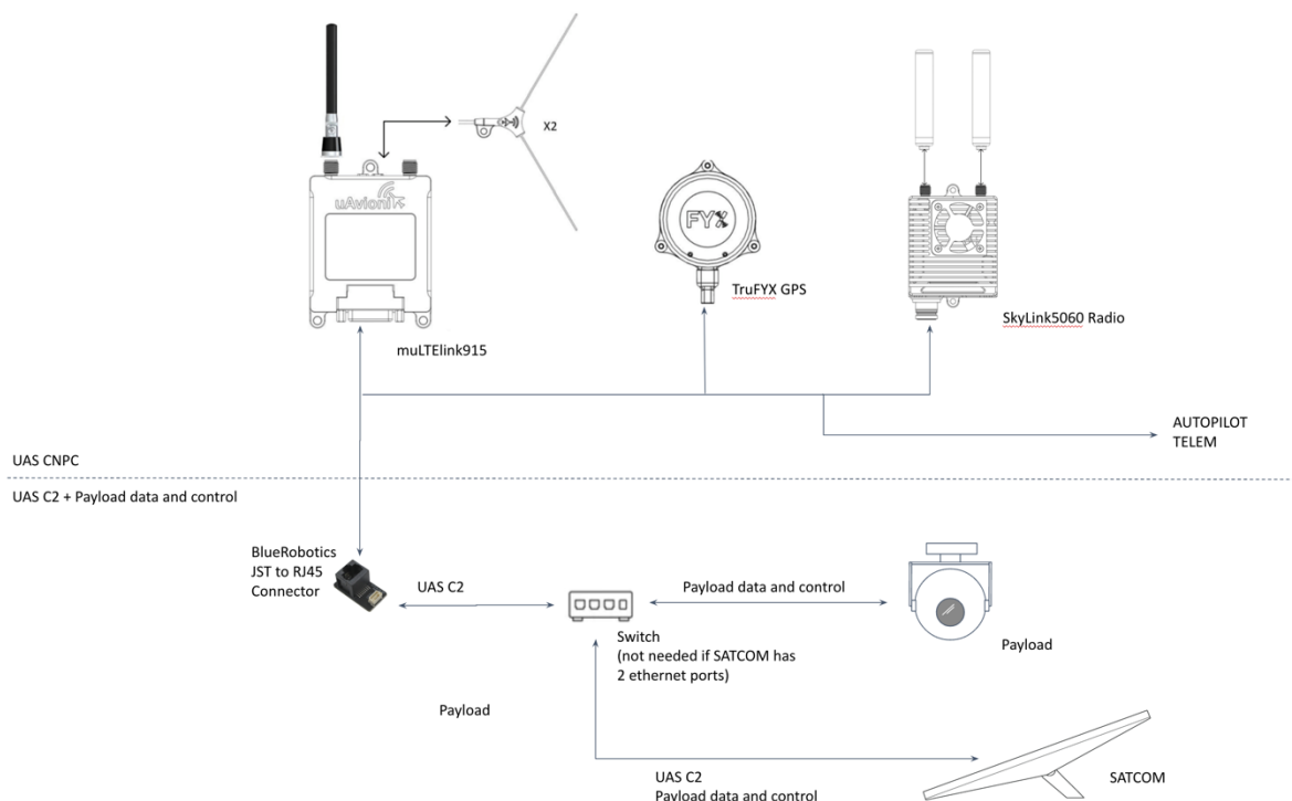
Figure 277: muLTElink Diagram with SATCOM Incorporating Payload Solution
