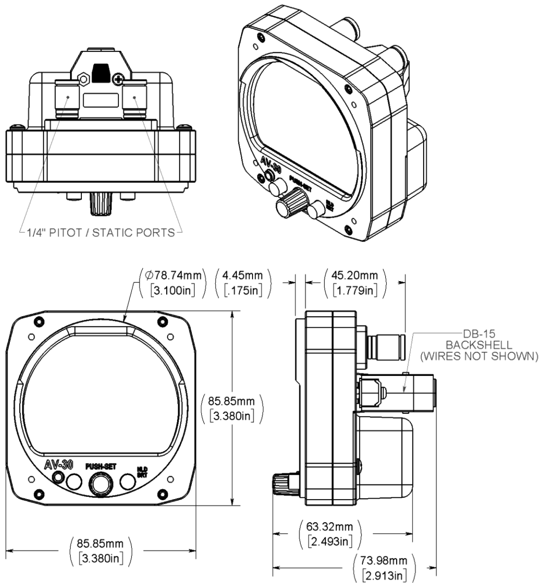
Figure 5 – Mechanical Drawing
