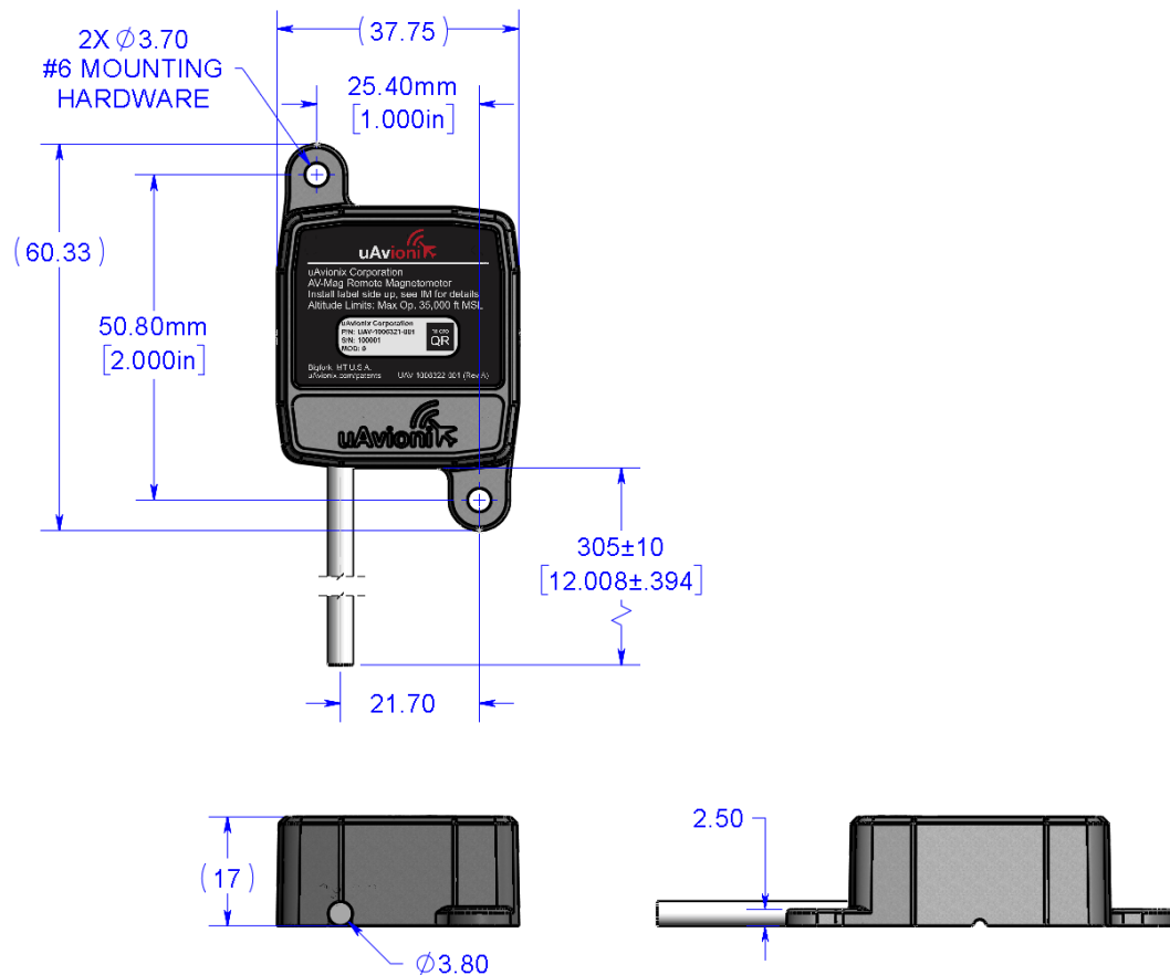
Figure 13 - AV-Mag Mechanical Drawing
