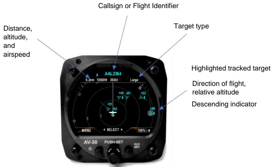
Figure 34 - Traffic Target Tracking Function
