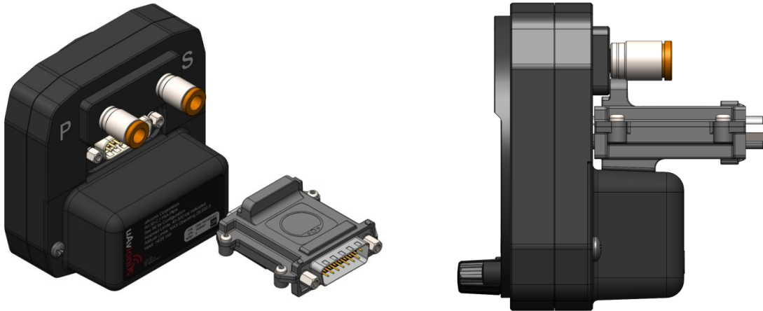
Figure 48 - AV-Link Attached to AV-30-C
