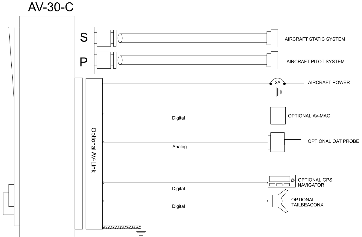
Figure 3 - AV-30-C Aircraft Systems Interfaces - DG Mode
