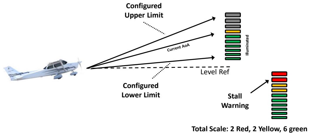
Figure 45 – AoA Upper and Lower Limits
