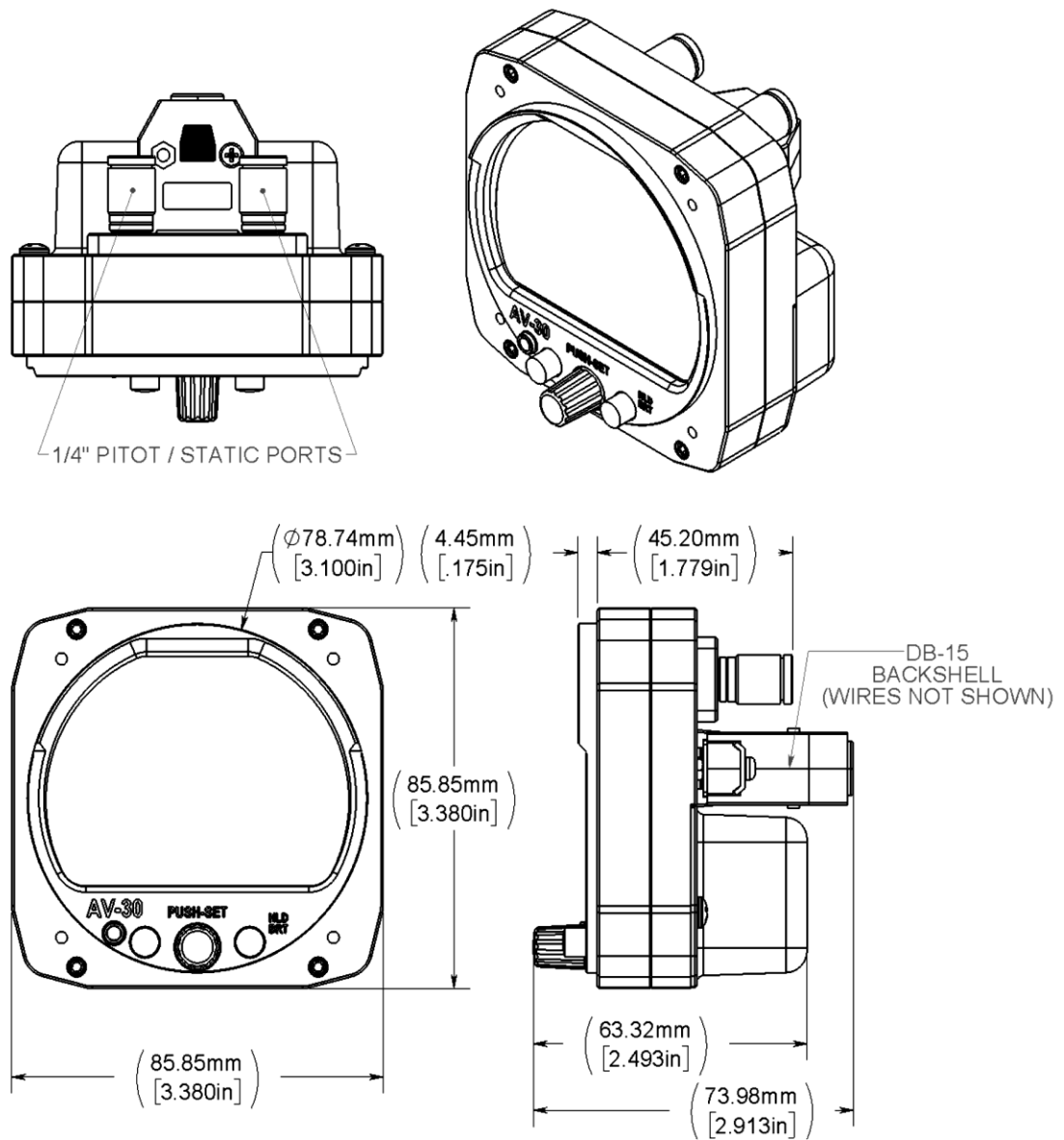
Figure 5 – Mechanical Drawing
